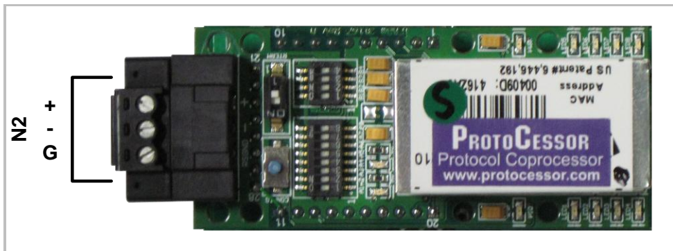
Figure 3: N2 Electrical Connections
